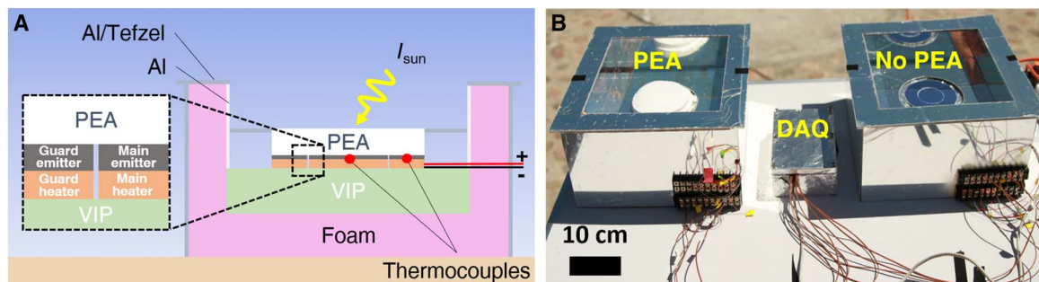
Fig. 4. Experimental setup. (A) Schematic of the radiative cooler. A PEA/emitter/heater assembly is placed on top of a vacuum insulation panel (VIP) that sits inside a thermally insulating foam (FOAMULAR 150) box. The box is covered with Tefzel-coated polished aluminum sheets to minimize solar heating. The emitter/heater consists of two separate parts—the main emitter/heater and the guard emitter/heater (see inset). (B) Picture of the setup consisting of two identical devices (left: device with PEA; right: device with no PEA). A DAQ (enclosed in an aluminum box) is also visible. More pictures showing details of the experimental location and setup are included in fig. S3. Photo credit: Arny Leroy, Massachusetts Institute of Technology.
