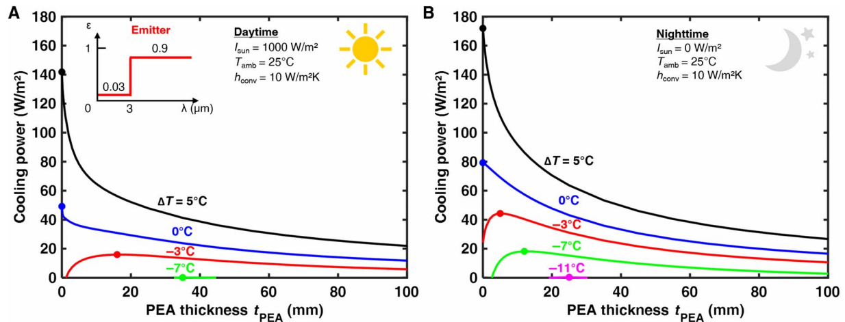
Fig. 3. Performance of radiative coolers with PEA. (A) Daytime cooling performance of a semi-ideal selective emitter ( R_{\text{solar}} = 1 - \alpha_{\text{solar}} = 0.97 and \epsilon_{\text{IR}} = 0.9 ) at different temperatures ( \Delta T = T_{\text{emitter}} - T_{\text{amb}} ). The maximum cooling power is shown by a solid point for each emitter temperature curve. An optimal aerogel thickness exists to achieve the maximum cooling power at a given emitter temperature. The results shown were calculated based on the U.S. Standard Atmosphere 1976. Atmospheric conditions specific to a location and time, such as humidity and cloud cover, can considerably affect the results and should be accounted for accordingly (19). (B) Results for nighttime cooling performance. Higher cooling power and lower emitter temperatures can be achieved due to the absence of solar irradiation.
