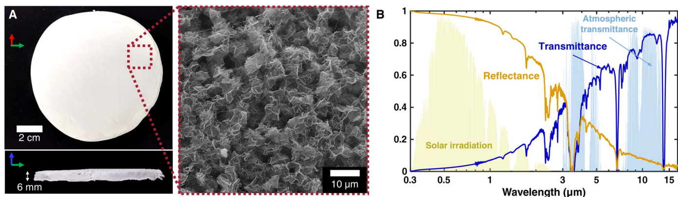
Fig. 2. Polyethylene aerogel. (A) Image of a 10-cm-diameter and 6-mm-thick PEA sample. The inset shows an SEM image at a magnification of \times 1500 . Photo credit: Arny Leroy, Massachusetts Institute of Technology. (B) Hemispherical transmittance and reflectance of a 6-mm-thick PEA sample along with the normalized AM1.5 solar spectrum and the atmospheric transmittance (U.S. Standard Atmosphere 1976).
