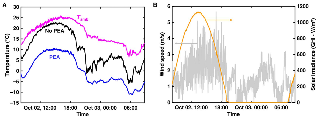
Fig. 5. Stagnation temperature of radiative cooler. (A) Stagnation temperature of two devices (12-mm-thick PEA and no PEA) over a 24-hour period in early October in San Pedro de Atacama, Chile. The device with the PEA achieves 13°C subambient cooling around solar noon (30-min average around 13:22; GHI = 1123 W/m 2 ) compared with 1.7°C without the PEA. (B) Wind speed and solar irradiation during the stagnation temperature experiment.
