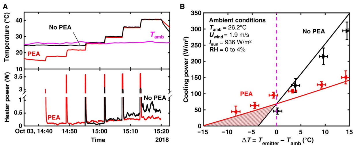
Fig. 6. Cooling performance of radiative cooler. (A) Measured emitter temperature of two devices (18-mm-thick PEA and no PEA) as well as the corresponding heater power and ambient temperature during the cooling power experiment. (B) Cooling power of the two devices as a function of the emitter subcooling in San Pedro de Atacama, Chile. The shaded area represents the range of cooling power and subambient temperatures made accessible by the PEA compared with an uninsulated emitter.
